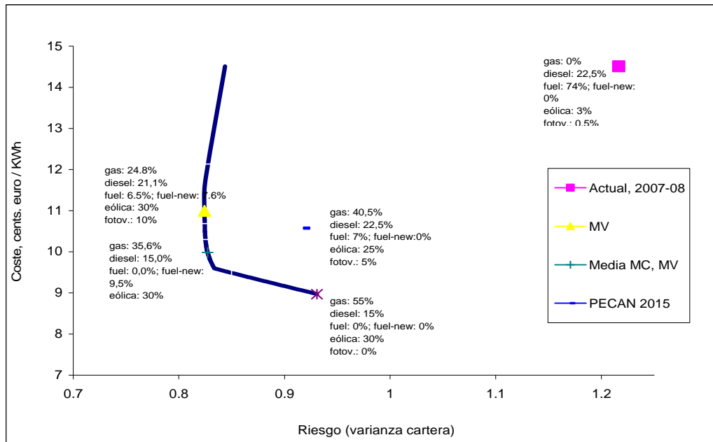
Figure 5. Efficient electricity generating frontier in the Canaries
