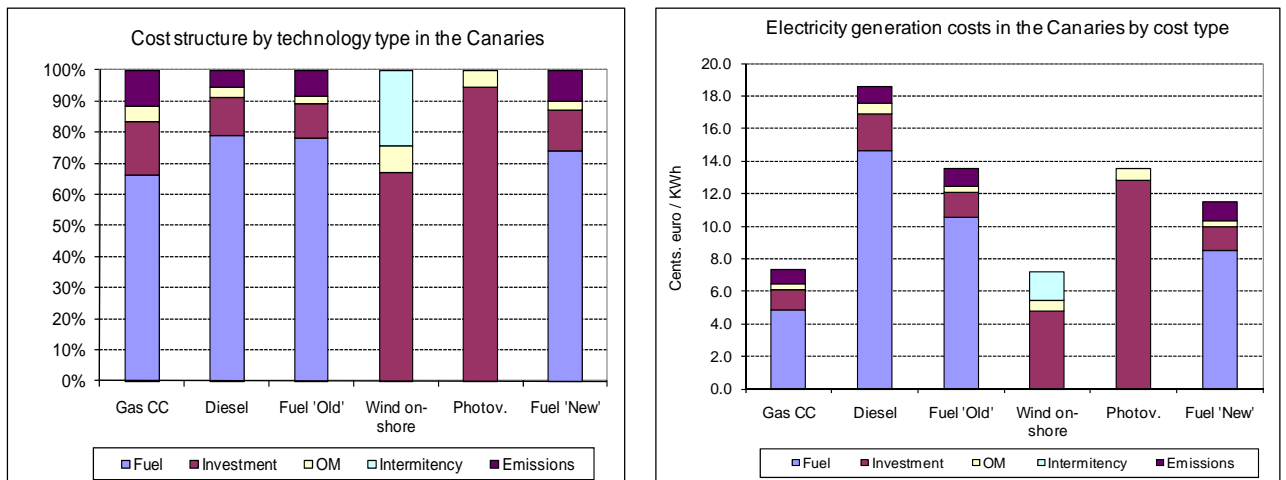
Figure 2. Electricity generation cost structure in the Canaries
